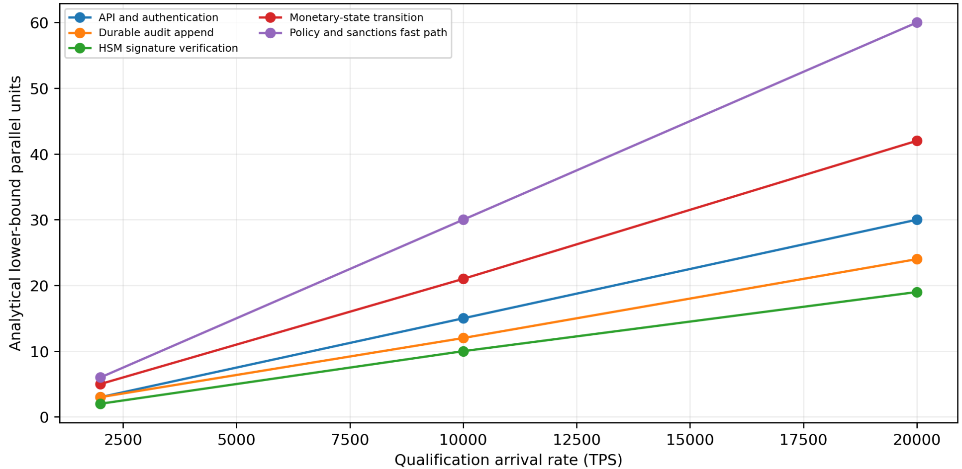
Necessary capacity lower bounds at 60% utilization and 2x headroom
