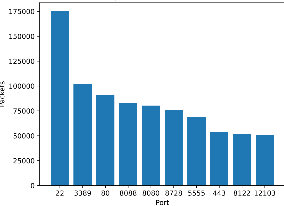
Top 10 Scanned Ports (TCP)
