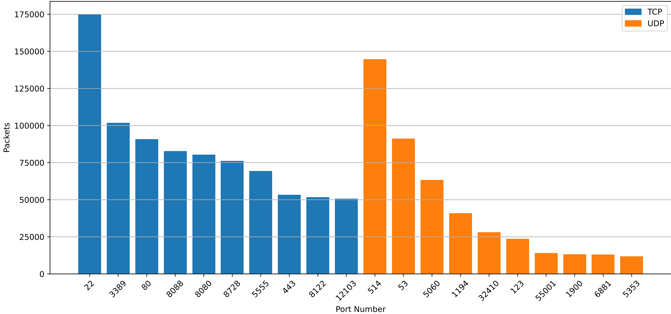
Top 10 Scanned Ports (TCP and UDP)
