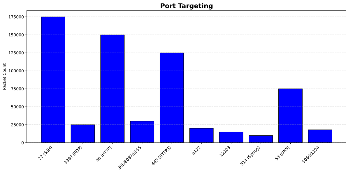
Figure 5: Port targeting by the top scanner IP
