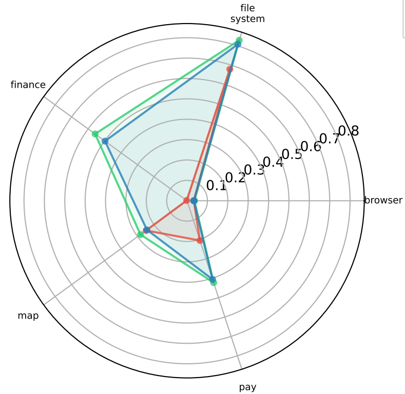
MCPToolBenchPP
