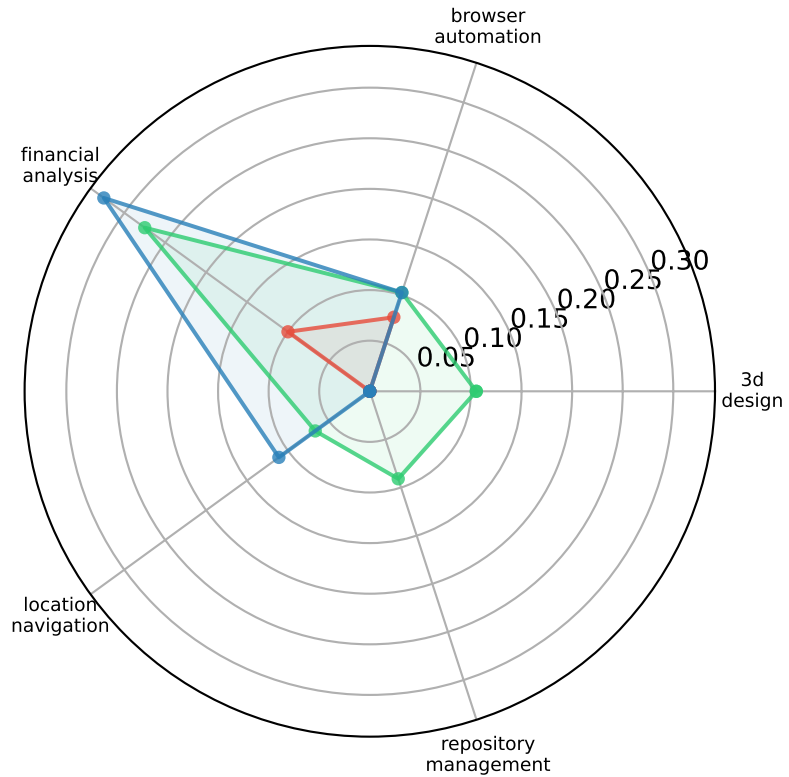
MCP-Univers
