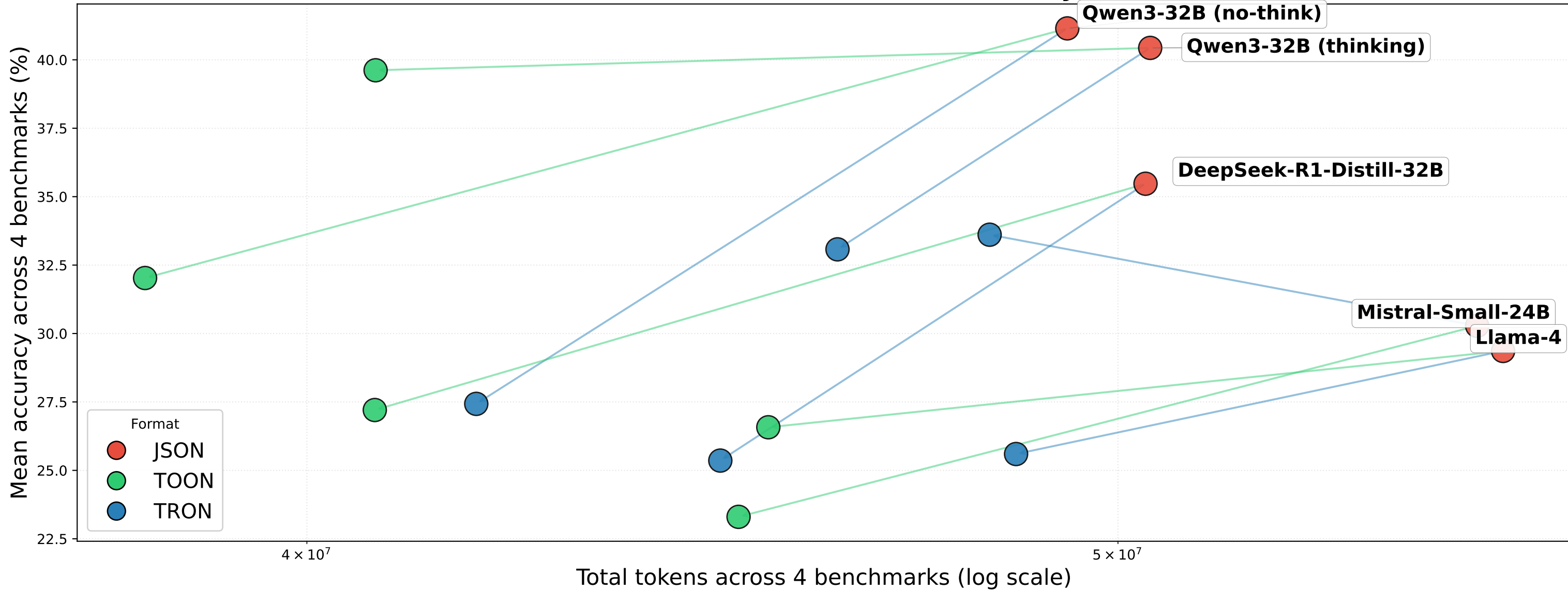
Per-model absolute token--accuracy
