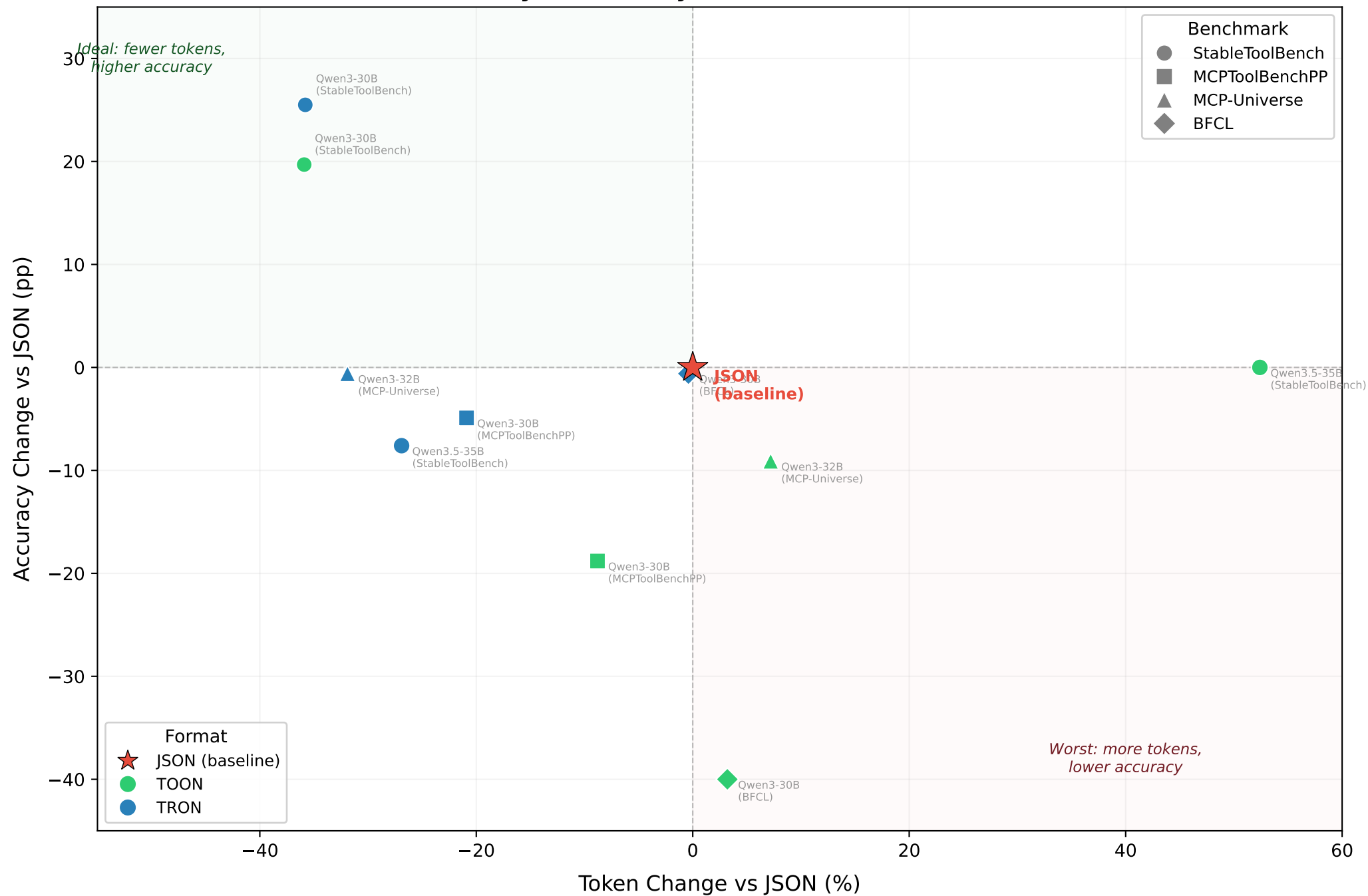
Token-Accuracy Tradeoff by Format, Model, and Benchmark
