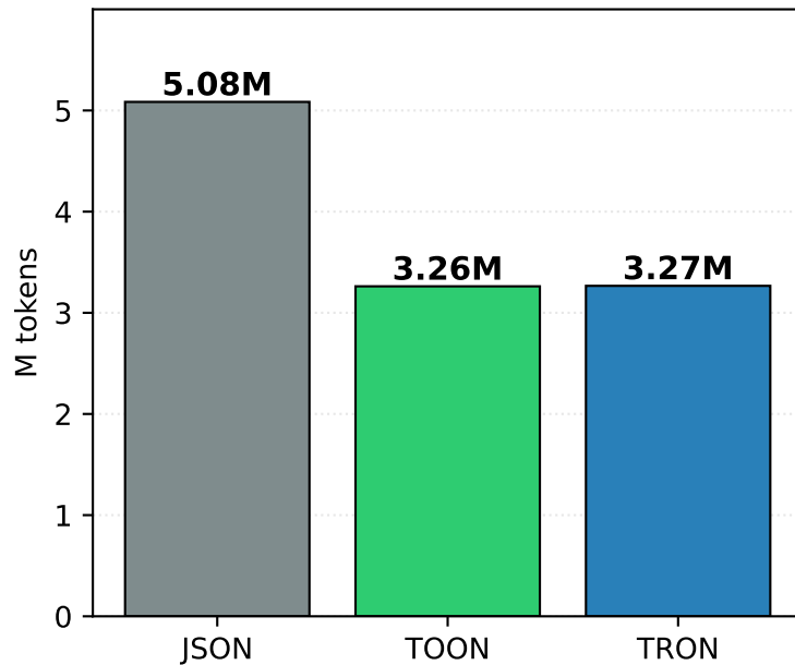
Total tokens
