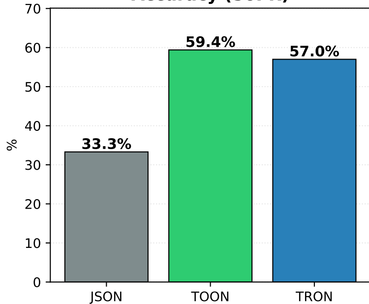
Accuracy (SoPR)
