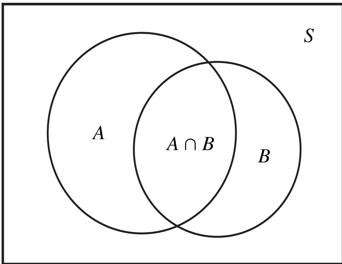
Figure 6: 文氏圖
