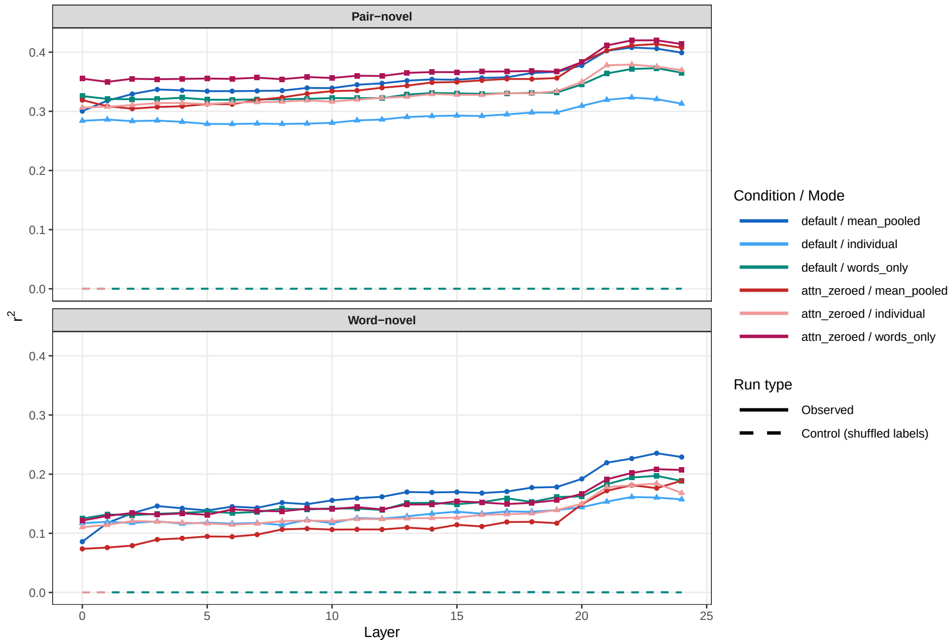
OPT-350m-20eps-seed964 — r^2 by layer
