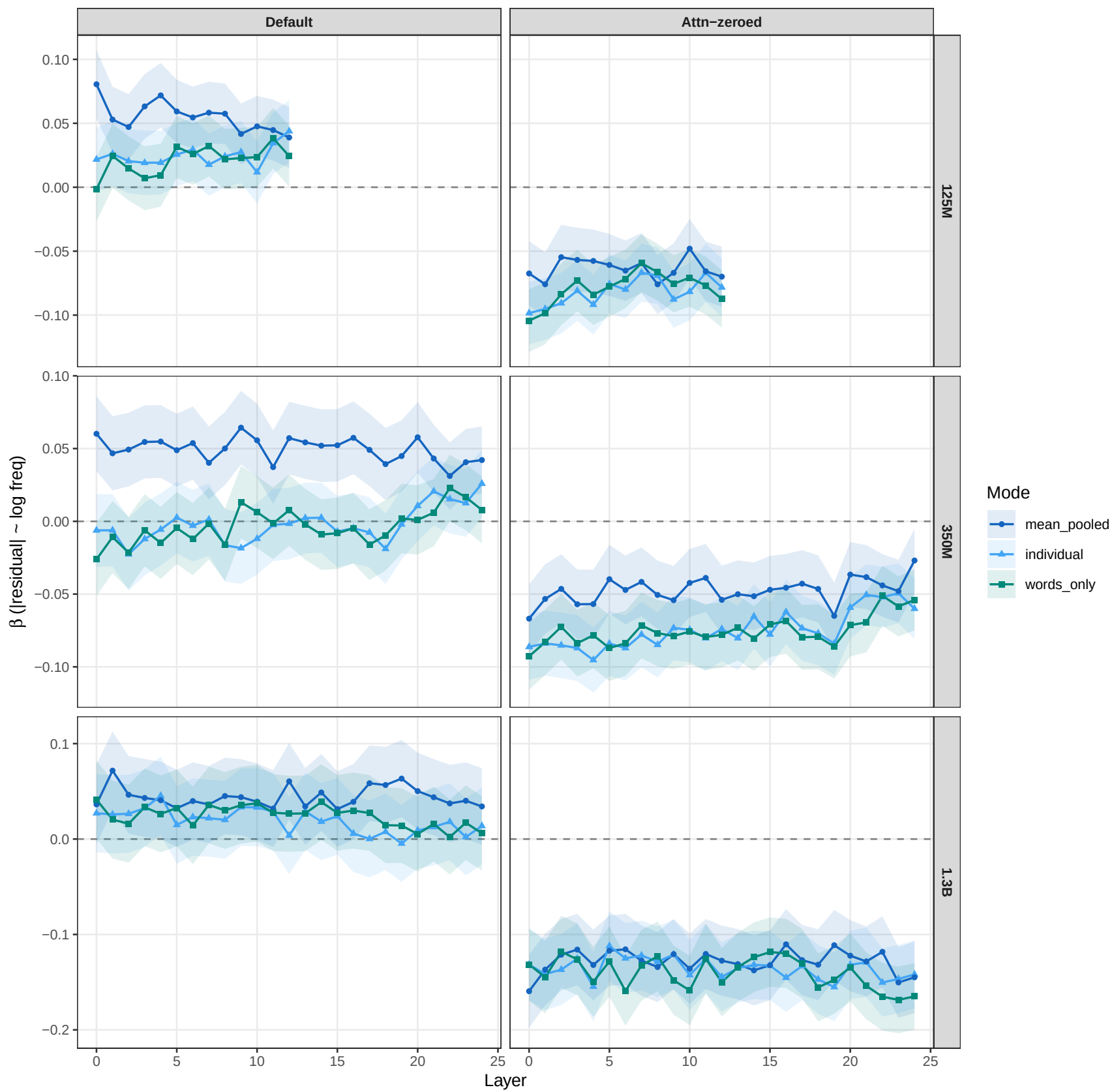
Corpus frequency regression — all models
