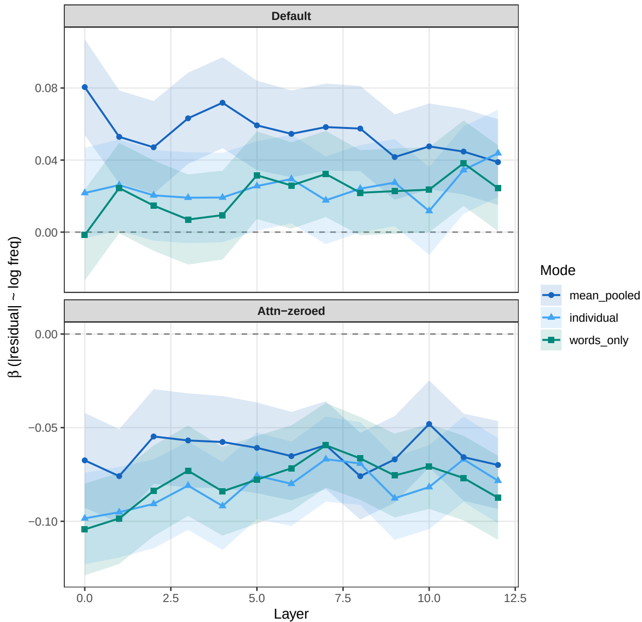
OPT-125M — corpus frequency regression by layer
