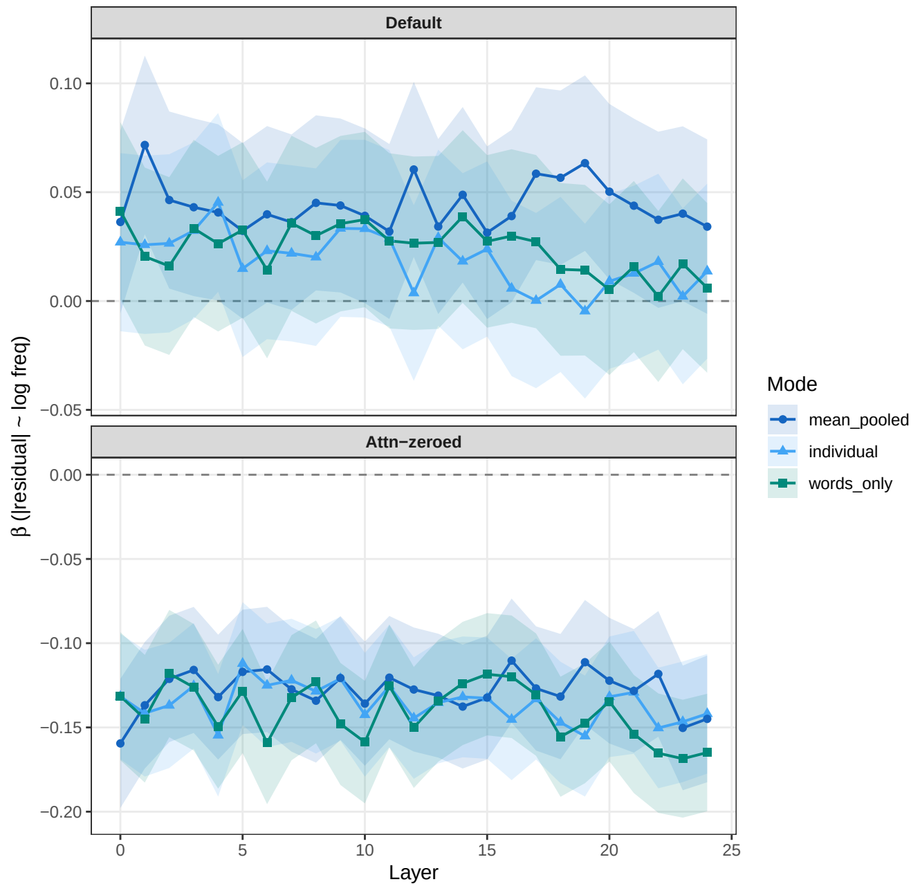
OPT-1.3B — corpus frequency regression by layer
