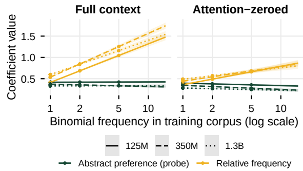
Figure 2: How strongly each source contributes to the BabyLM models' ordering preference, by binomial frequency. Values are slopes from the fitted posteriors of Equation 1. Bands are 95% credible intervals.
