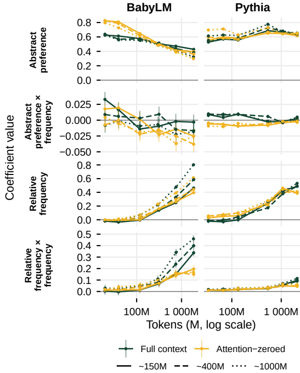
Figure 6: All four terms of Equation 1 across training, with 95% credible intervals. Rows are the two sources and their interactions with overall frequency; color marks the attention condition and linetype the model size.
