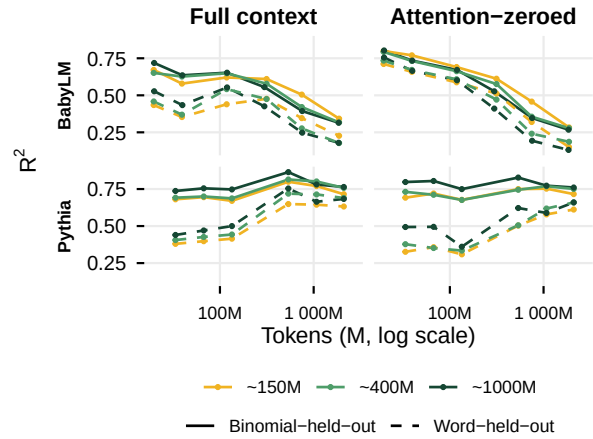
Figure 5: Cross-validated probe R^2 across BabyLM and Pythia training checkpoints, by attention condition and cross-validation split. Control R^2 \approx 0 .
