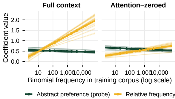
Figure 4: How strongly each source contributes to the ordering preference, by binomial frequency, for the 13 large-scale models. Values are simple slopes from the fitted posteriors of Equation 1. Faint lines are individual models with their 95% credible intervals, bold lines their mean.
