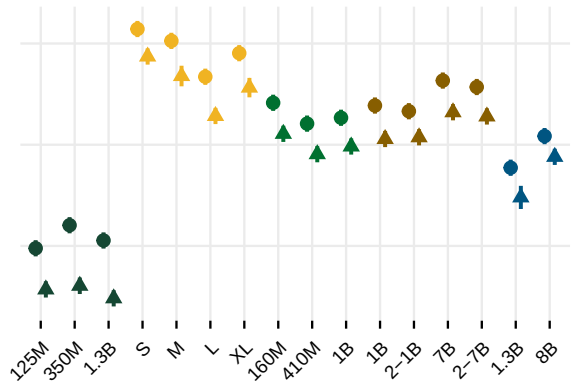
Attention-zeroed
