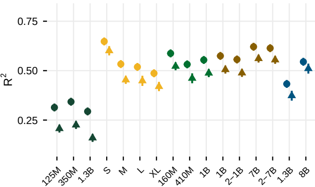
Full context
