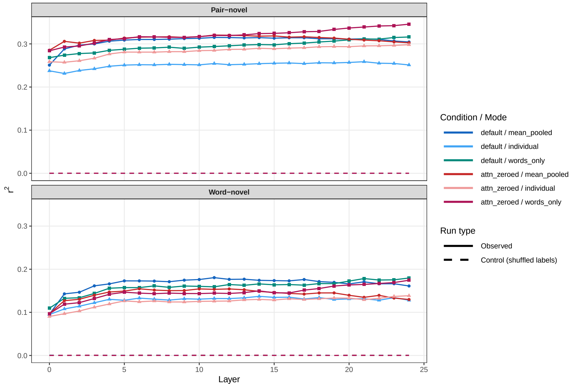
OPT-1_3b-20eps-seed964 — r^2 by layer
