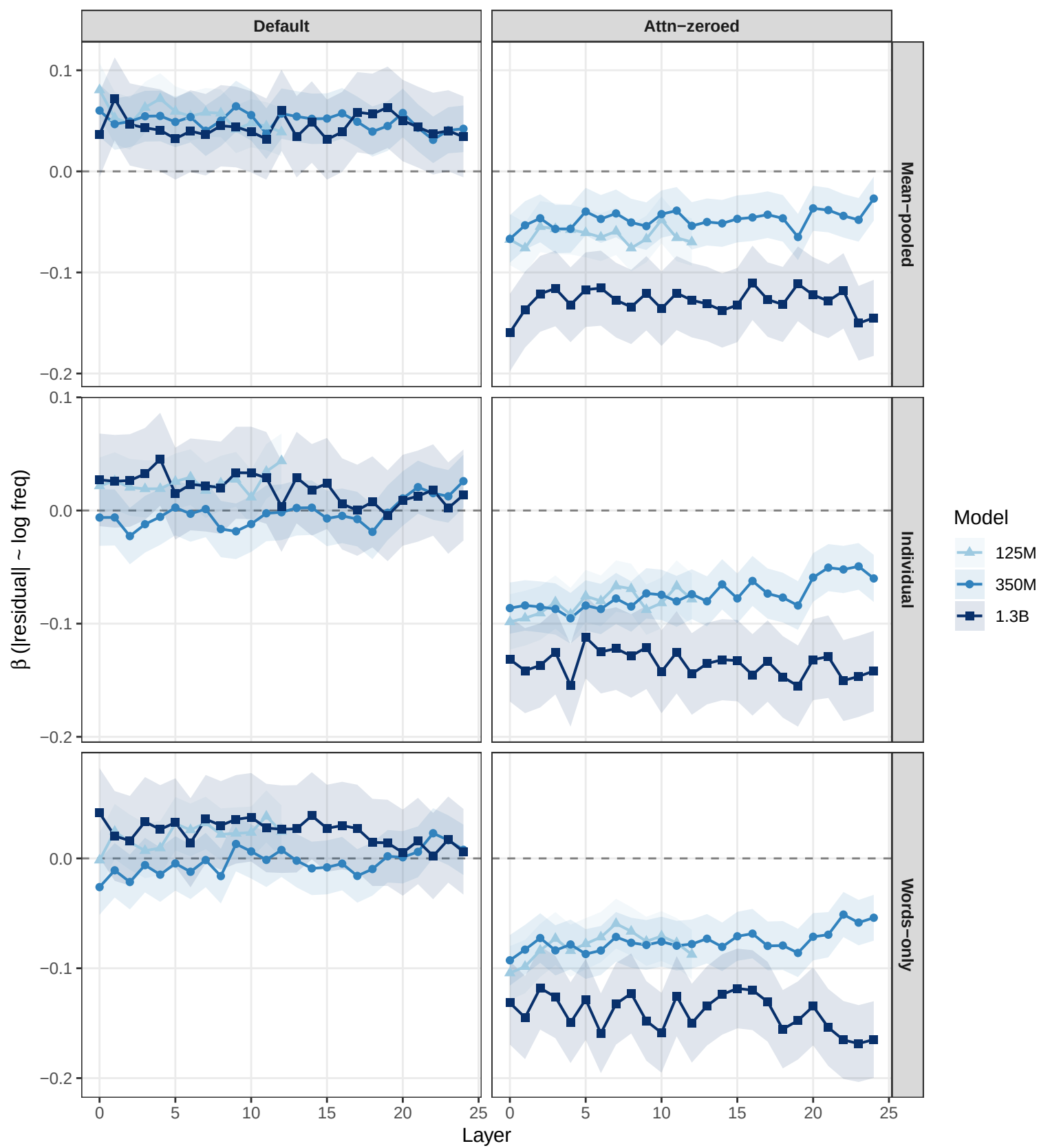
Corpus frequency regression by model size
