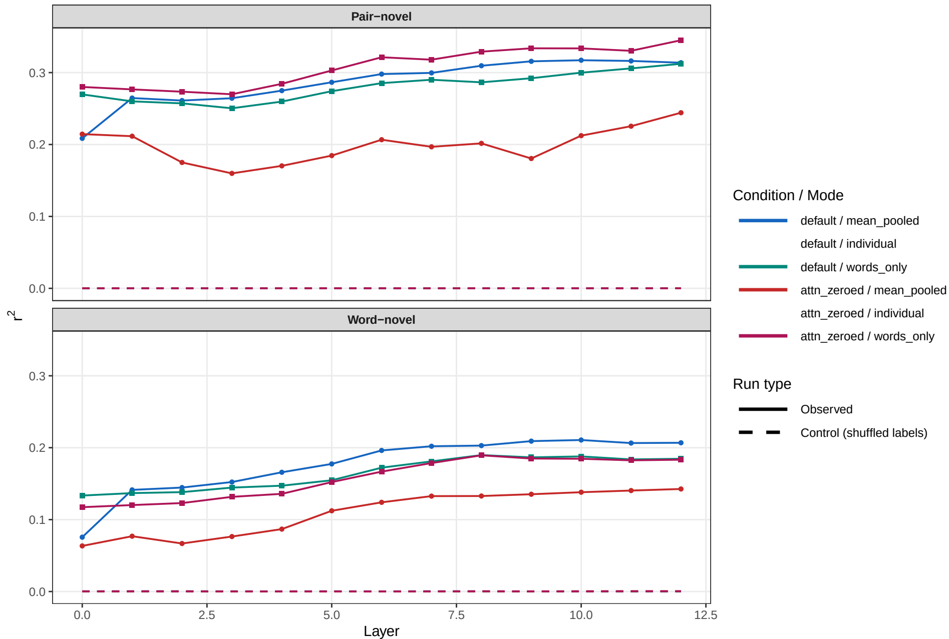
OPT-125m-20eps-seed964 — r^2 by layer
