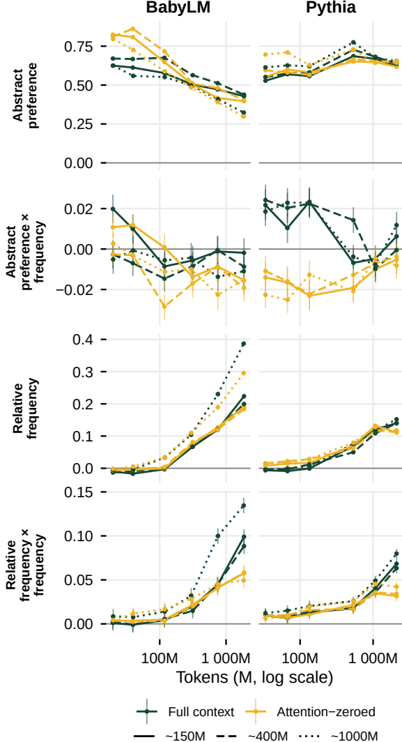
Standardized slope on ordering preference
