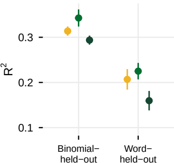
Full context
