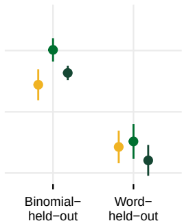
Attention-zeroed
