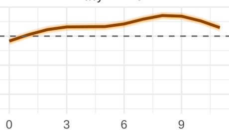
BabyLM 125M
