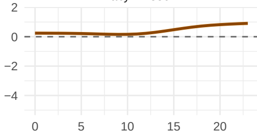
BabyLM 350M
