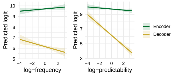
Figure 5: Final-layer brms predicted logit by frequency (left) and predictability (right) for Whisper encoder and decoder. Lines and bands as in Figure 1.
