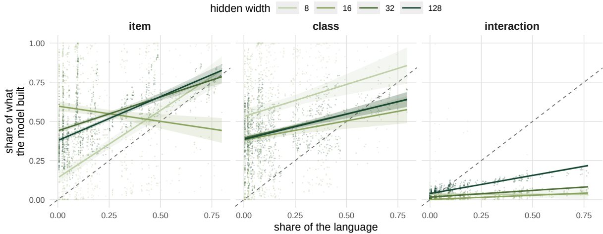
Figure 3: What the learner builds of each component, against how much of that component the language held, under ReLU. Each faint point is one run. Horizontally it sits at that component’s share of the training distribution, alongside the other two and the context; vertically at the same component’s share of the item-by-class structure the model built. Lines are least-squares fits through the runs at each hidden width, with their 95% bands. The dashed diagonal is where a representation would sit that reproduced the language’s composition exactly: above it a component is built up beyond what the language asked for, below it the component is held back. Runs in which none of the three components had a re-split 95% interval excluding zero are not plotted, since the three shares then divide noise; all such runs are at width 8, and their number is given in the text.
