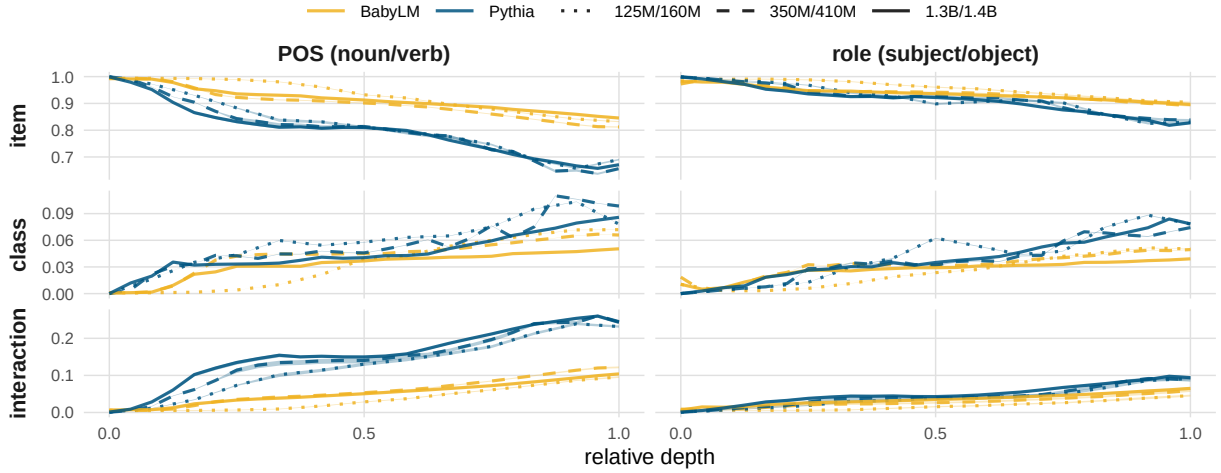
Figure 4: The three components through the network, for every model and linguistic category. Relative depth runs from the static embedding layer (0) to the final block (1). Rows are the item effect, the class effect and their interaction, each as a share of the item-by-class structure, which sum to one within each model and layer. Each line is one model: color distinguishes the training corpus, linetype the three matched widths. The shaded band is that model’s re-split 95% interval.
