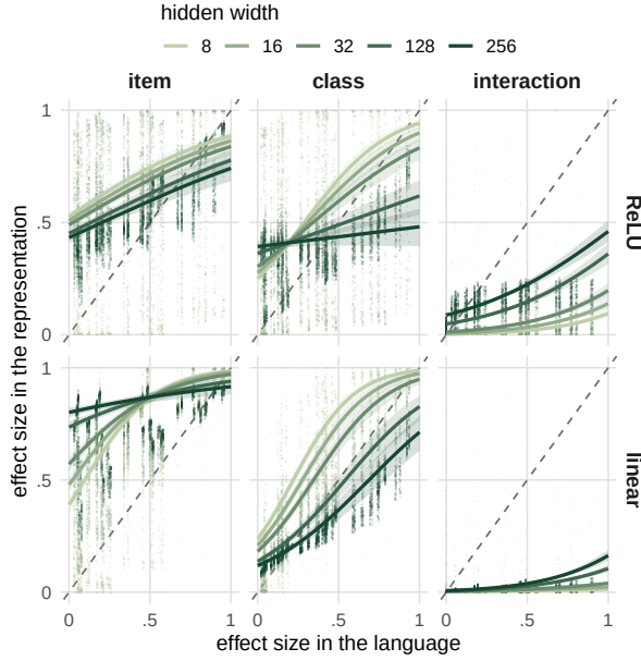
Figure 3: Each component’s share of the representation against its share of the language, by activation. Faint points are runs; lines are fitted values from Equation 3 with 95% intervals, at the mean of the other two effect sizes and of the interaction’s rank. The dashed diagonal is exact reproduction of the language’s composition. Runs in which no component’s re-split interval excluded zero are not plotted.
