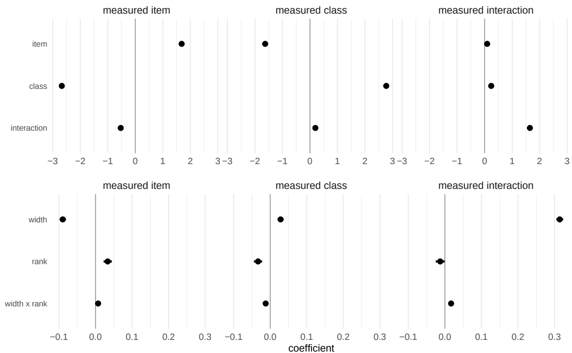
Figure 8: Coefficient estimates from the size model (Equation 3), one panel per measured component. The upper block holds the planted effect sizes and the lower the architecture terms, which are on a much smaller scale and so are drawn on their own axis. Points are posterior medians with 95% intervals.
