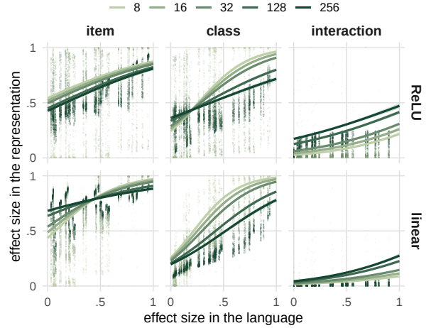
Figure 3: Ground-truth effect size of each component in the language (x) against its size in the MLP’s representations (y). Points are runs; lines are fitted values from the size model (Equation 3) with 95% intervals, colored by hidden width.
