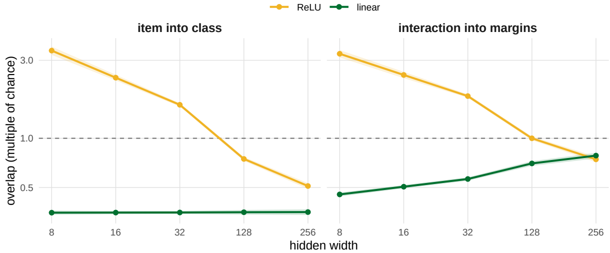
Figure 10: Two overlap measurements as a function of width of the hidden layer. Left: the item effect projected onto the class direction. Right: the interaction projected onto the span of both margins. The dashed line is chance.
