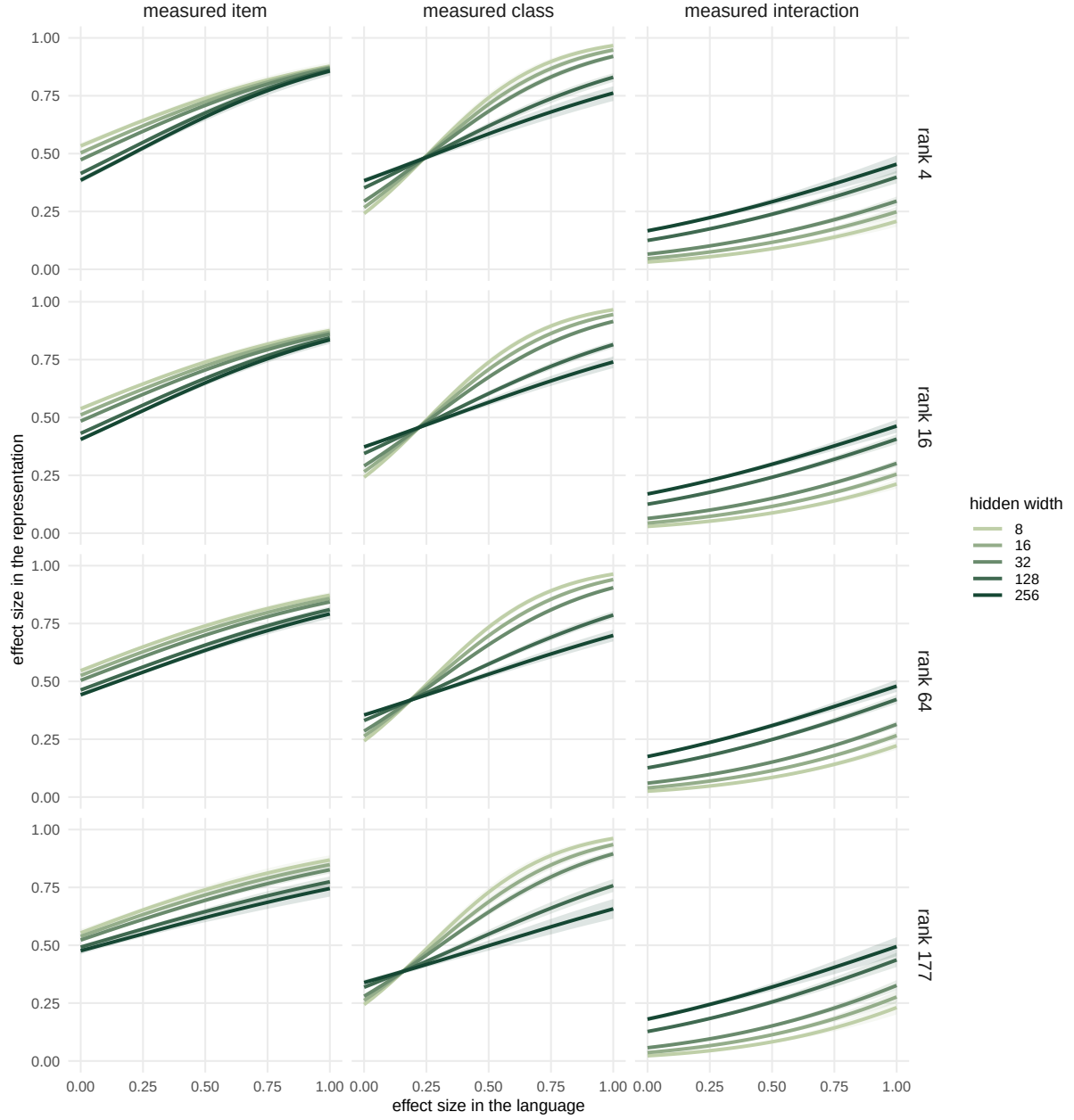
Figure 9: Model results for the size model (Equation 3). Columns are the three measured components, rows are the planted interaction rank, and lines are hidden widths, with 95% intervals. Holding rank fixed within a row is what separates the width effect from the width-by-rank term; the near-identical rows show how little the rank changes it.
