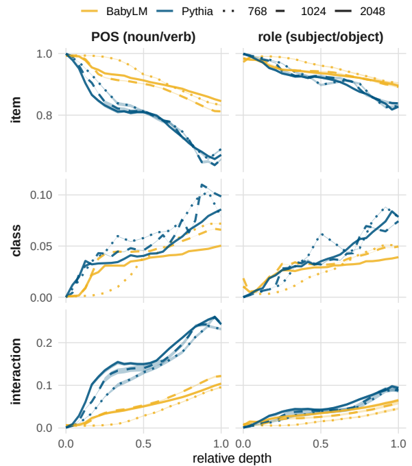
Figure 4: The three components through the network, by linguistic category. x-axis is relative depth, from the static embedding layer (0) to the final block (1). The y-axis is each component’s share of the item-by-class structure: item, class, and their interaction. Each line is one model: color is the training corpus, linetype the hidden width; the band is that model’s re-split 95% interval.
