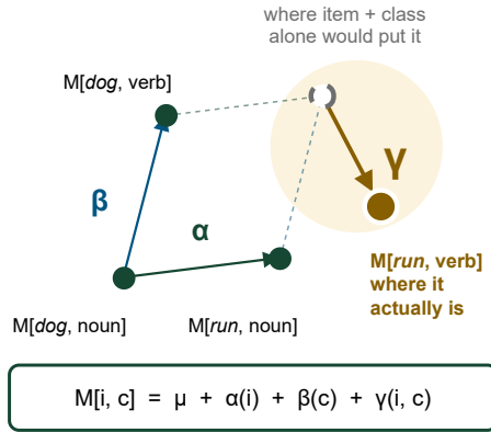
Figure 2: The four item-by-class means formed by two items in two classes. Under an item part plus a class part, three corners fix the fourth and the parallelogram closes. The arrow is \gamma(i, c) , the displacement between the fourth mean and the point that additive account places it at, with length \|\gamma(i, c)\| .
