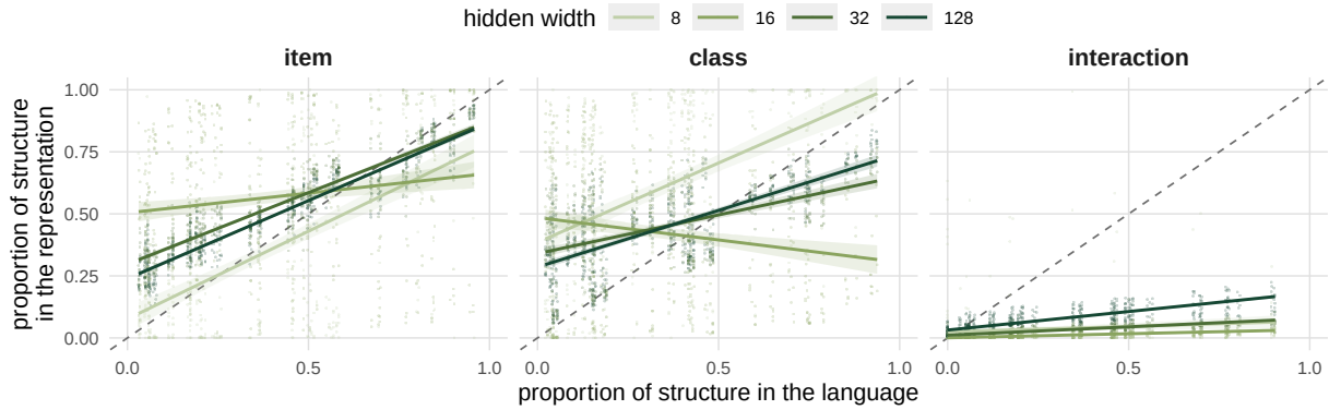
Figure 3: What the model represents of each component, against how much of that component the ground-truth language held, under ReLU. Each faint point is one run. Lines are least-squares fits through the runs at each hidden width, shaded with a 95% confidence band on the fit. The dashed diagonal is where a representation would sit had it reproduced the language’s composition exactly. Runs in which none of the three components had a re-split 95% interval excluding zero are not plotted, since the three shares then divide noise.
