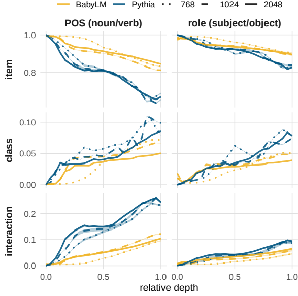
Figure 4: The fraction of the representation (ignoring context) accounted for by each component, such that they sum to 1, as a function of layer. x-axis is relative depth, from the embedding layer (0) to the final layer (1). The y-axis is the fraction of the representation accounted for by each component. Each line is one model, color is the training corpus, linetype is the hidden layer’s width; shading is the 95% interval.
