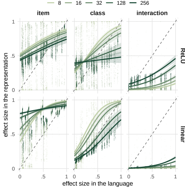
Figure 3: The x-axis is the ground truth effect size of each component in the language. The y-axis is the effect size of each component in the MLP’s learned representations. Points are individual runs; lines are fitted values from Equation 3 with 95% intervals, coloured by hidden width. The dashed diagonal indicates where representations matching the ground truth would lie.
