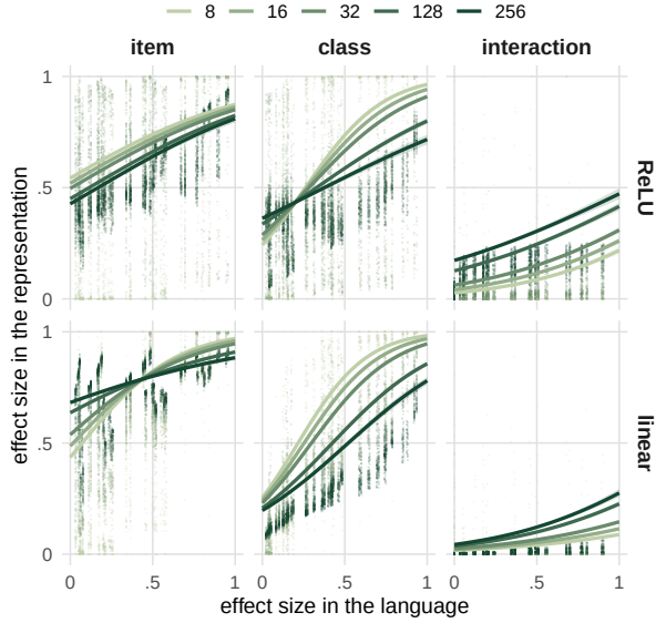
Figure 3: Ground-truth effect size of each component in the language (x) against its size in the MLP’s representations (y). Points are runs; lines are fitted values from the size model (Equation 3) with 95% intervals, colored by hidden width.
