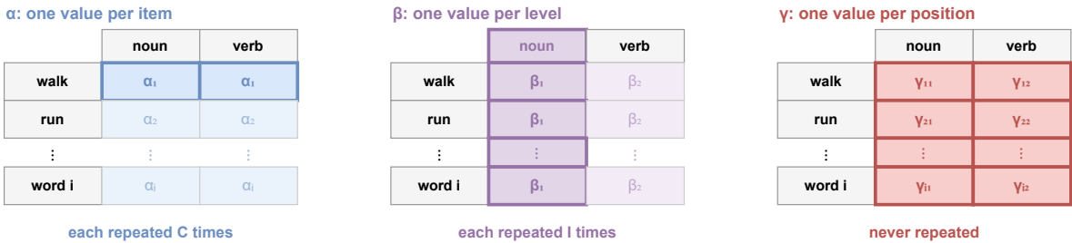
Figure 7: The three components across the grid of words and classes. An item effect is one value per word, the same in every class; a class effect is one value per class, the same for every word; and the interaction differs for every word in every class.
