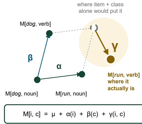
Figure 2: The four item-by-class means formed by two items in two classes. The arrow is \gamma(i, c) .
