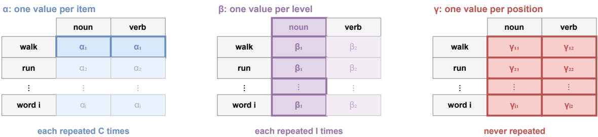
Figure 7: The three components across the grid of words and classes. An item effect is one value per word, the same in every class; a class effect is one value per class, the same for every word; and the interaction differs for every word in every class.
