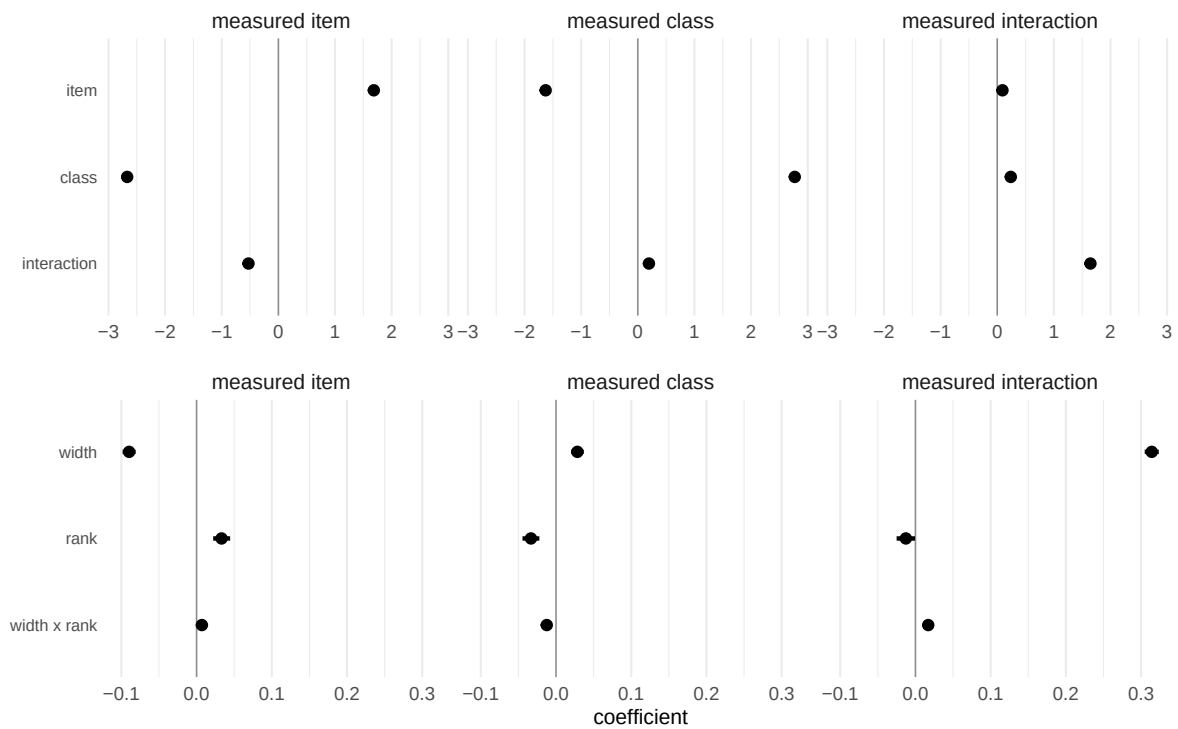
Figure 8: Coefficient estimates from Equation 3, one panel per measured component. The upper block holds the planted effect sizes and the lower the architecture terms, which are on a much smaller scale and so are drawn on their own axis. Points are posterior medians with 95% intervals.
