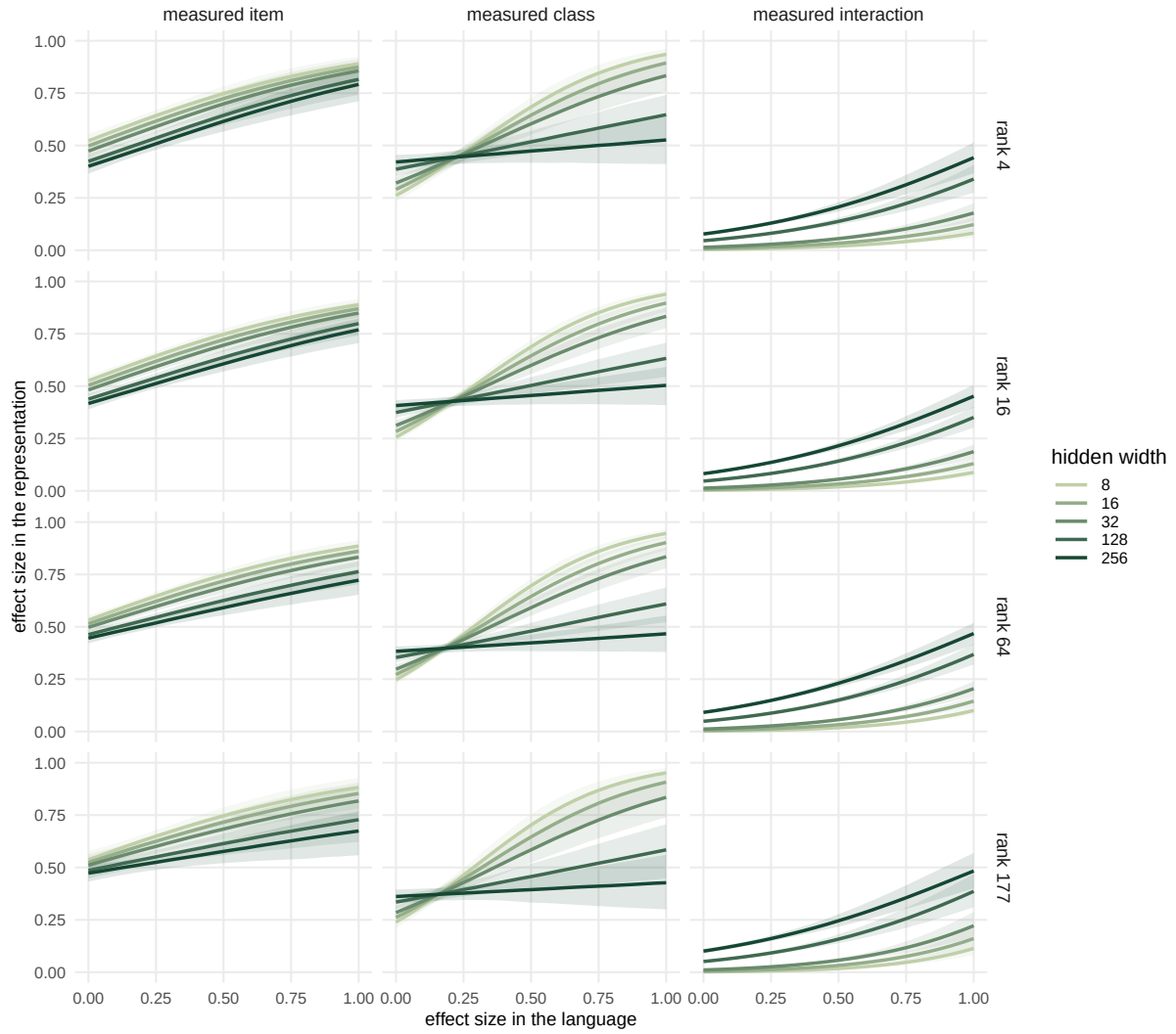
Figure 9: Model results for Equation 3. Columns are the three measured components and lines are hidden widths, with 95% intervals.
