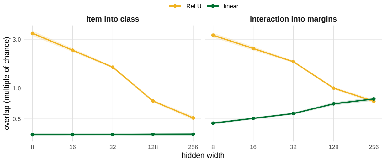
Figure 10: Two overlap measurements as a function of width of the hidden layer. Left: the item effect projected onto the class direction. Right: the interaction projected onto the span of both margins. The dashed line is chance.
