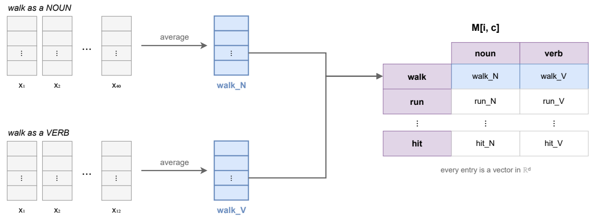
Figure 6: Each word in each class is observed in many contexts, and those observations are averaged to give that word’s representation in that class. Every one of these averages is a vector in \mathbb{R}^d , and every item appears in every class.
