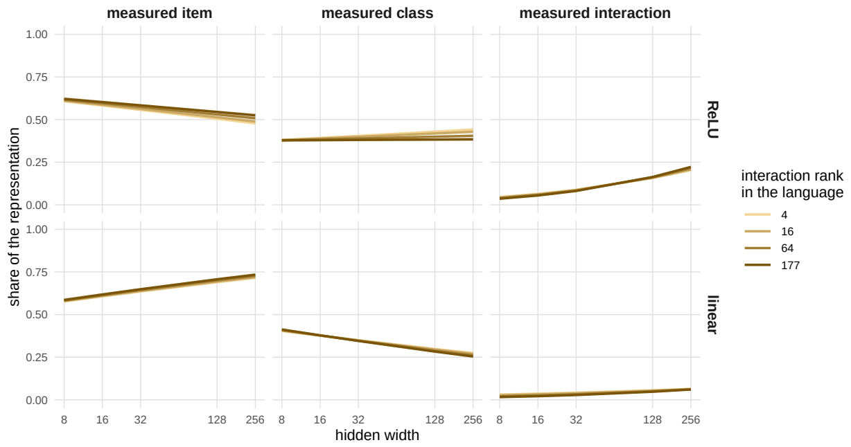
Figure 11: Fraction of the representation by each component (such that they sum to 1), against hidden width, with one line per rank of the interaction planted in the language and 95% intervals.
