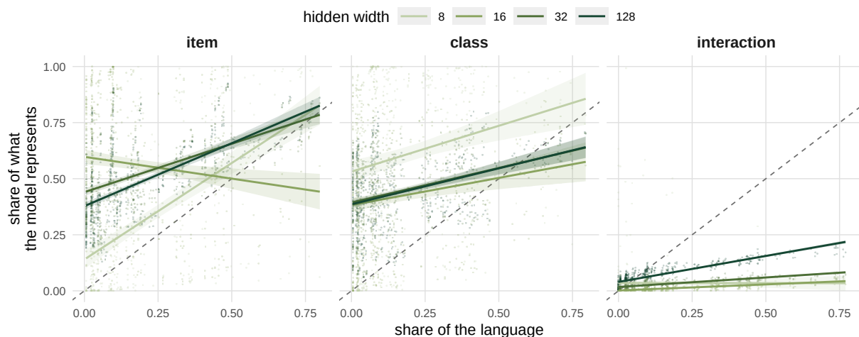
Figure 3: What the learner represents of each component, against how much of that component the language held, under ReLU. Each faint point is one run. Horizontally it sits at that component’s share of the training distribution, alongside the other two and the context; vertically at the same component’s share of the item-by-class structure the model represents. Lines are least-squares fits through the runs at each hidden width, with their 95% bands. The dashed diagonal is where a representation would sit that reproduced the language’s composition exactly: above it a component is over-represented relative to the language, below it under-represented. Runs in which none of the three components had a re-split 95% interval excluding zero are not plotted, since the three shares then divide noise; all such runs are at width 8, and their number is given in the text.
