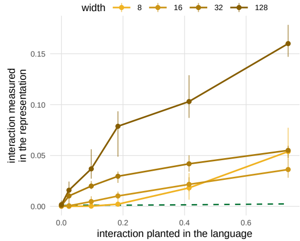
Figure 3: Measured interaction against the interaction planted in the language, over the 7,560 artificial-language runs. One line per hidden width under ReLU; the dashed line is the linear condition pooled over widths. Each point is the median over the runs in its bin, with their interquartile range. Both axes are shares of the whole: the planted share is the interaction's share of the target distribution alongside the item, the class and the context, and the measured share is its share of the representation, the grid's share of the representation times the interaction's share of the grid.
