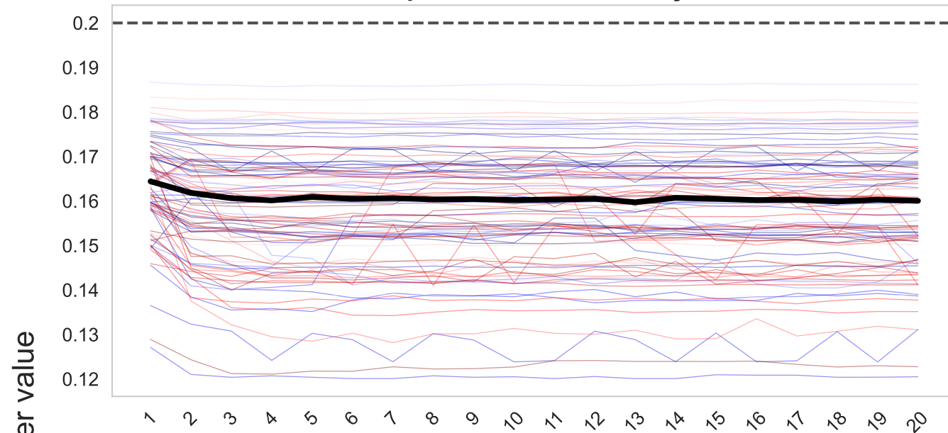
Variant Allele Frequency f_0
