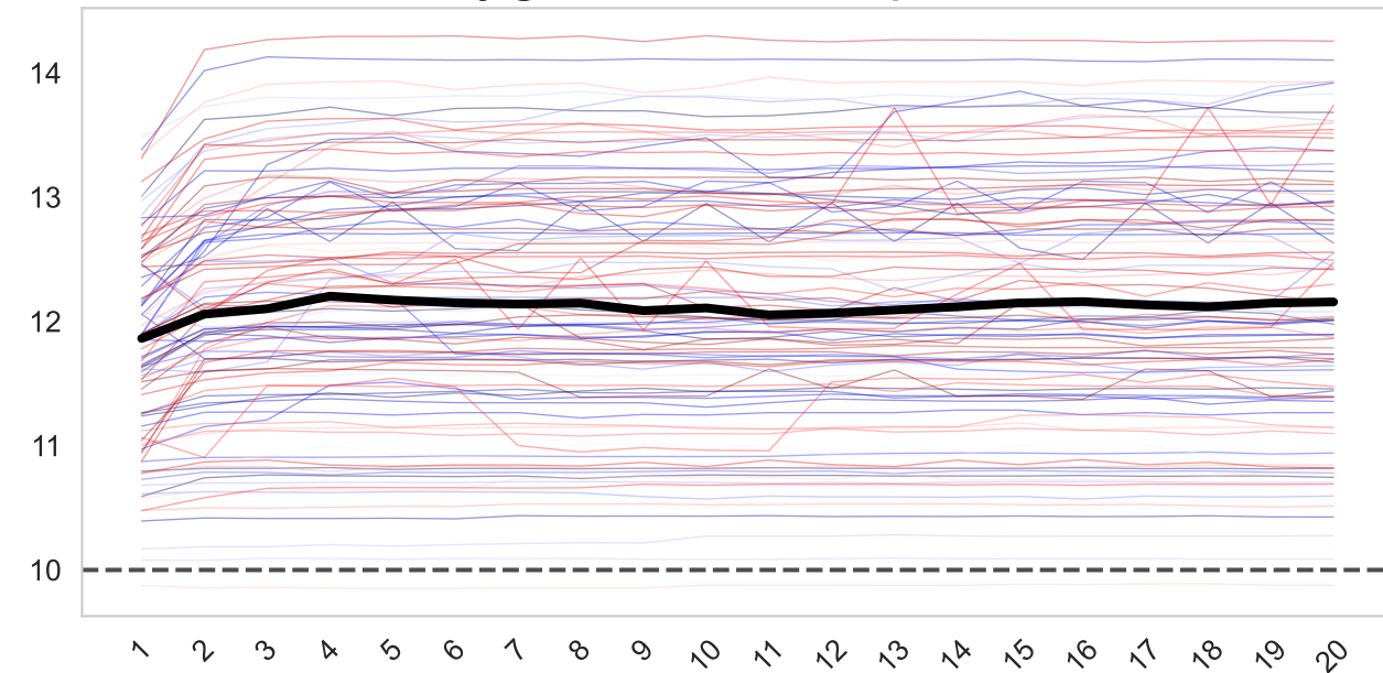
Heterozygous Overdispersion \omega_1
