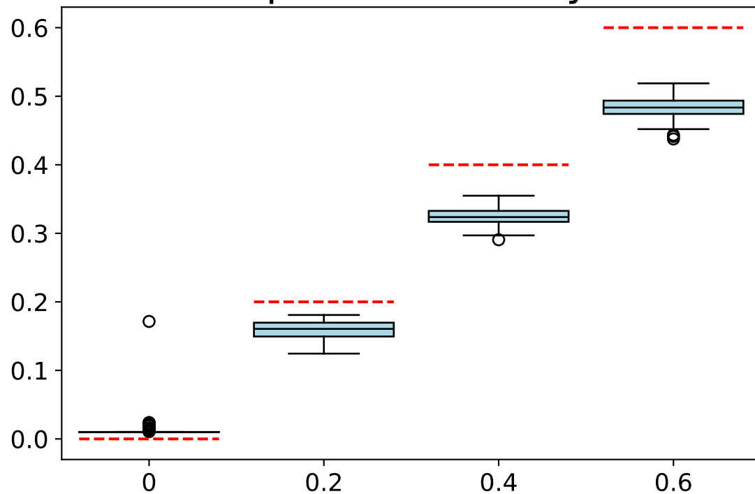
Variant Allele Frequency f_0
