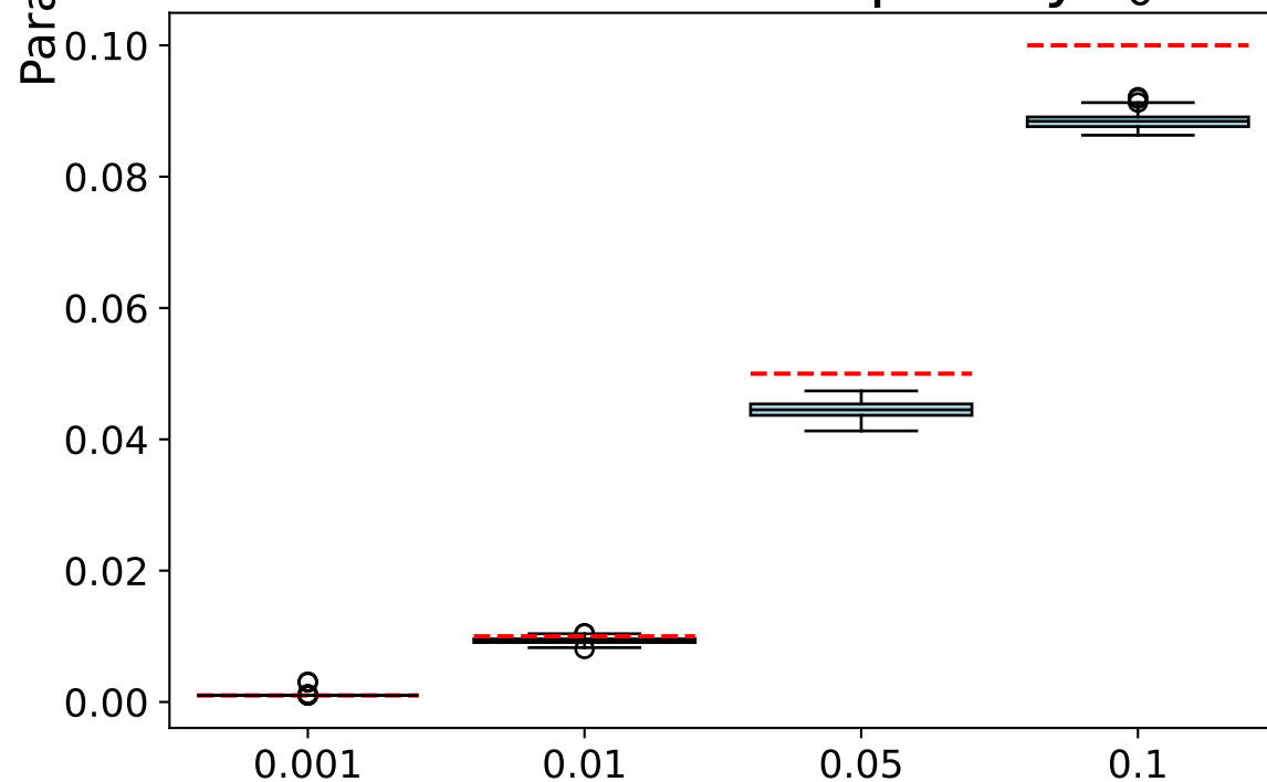
Variant Allele Frequency f_0
