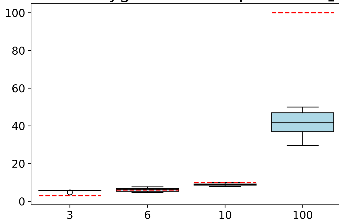
Heterozygous Overdispersion \omega_1
