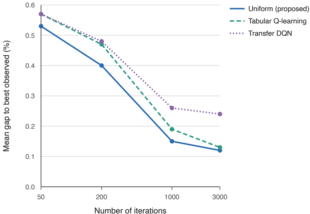
Learned policies never beat uniform
