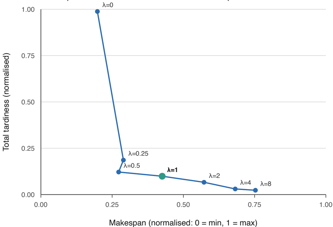
\lambda=1 keeps tardiness near-minimal at a moderate makespan cost
