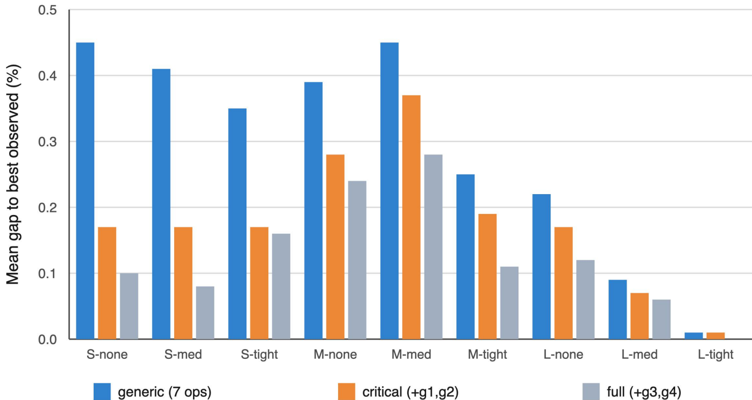
Adding bottleneck-guided operators lowers the gap in every cell (generic \geq critical \geq full)
