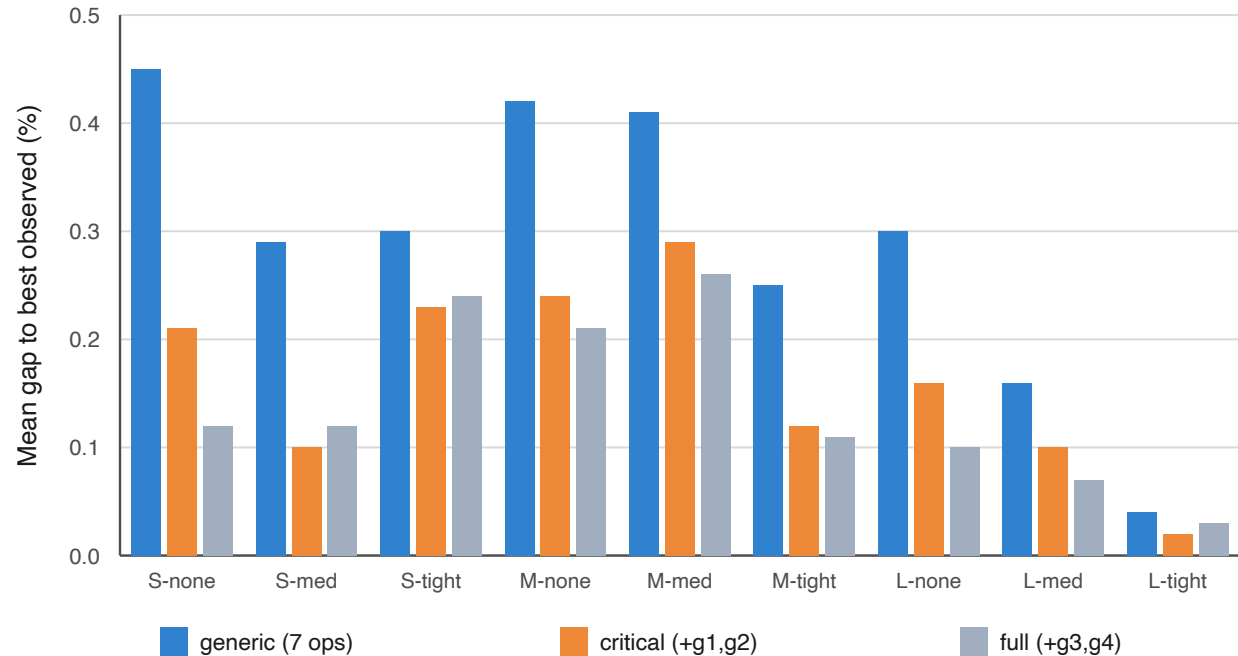
Guided operators g1, g2 lower the gap in every cell; g3, g4 add little
