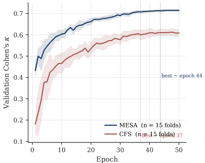
Validation \kappa across training
