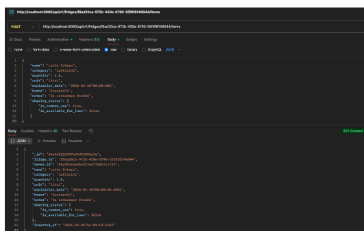
Figura 7.12: POST /api/v1/fridges/:id/items
