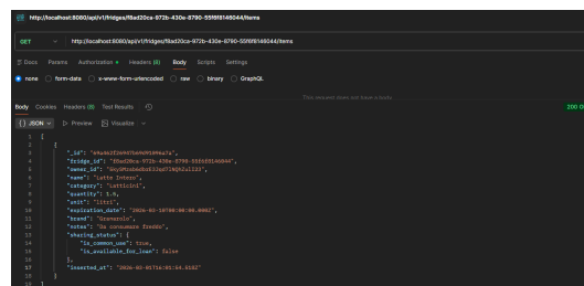
Figura 7.15: GET /api/v1/fridges/:id/items
