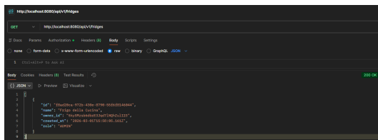
Figura 7.14: GET /api/v1/fridges
