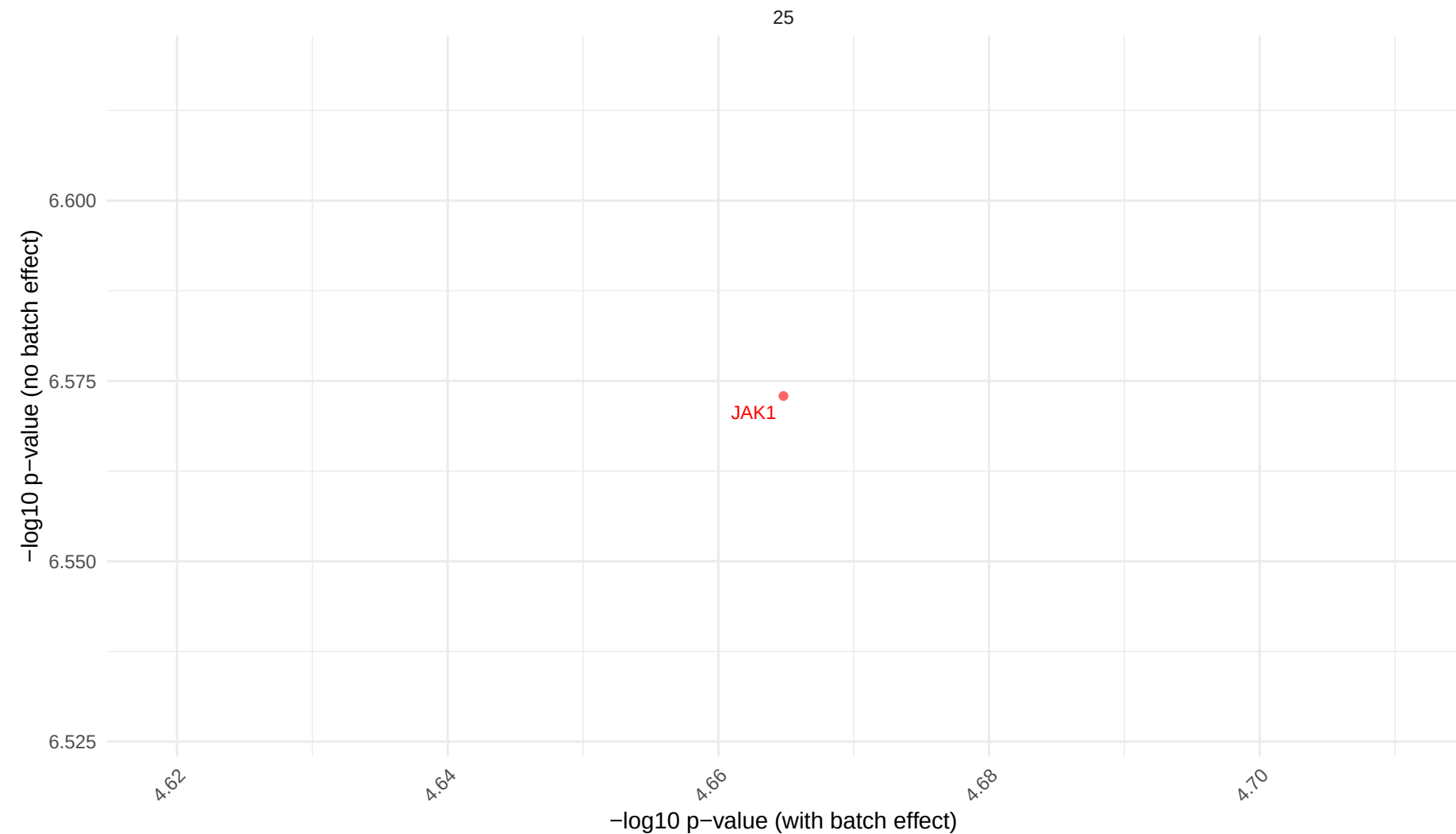
WT vs Mild: Batch vs No Batch (by Experiment)
