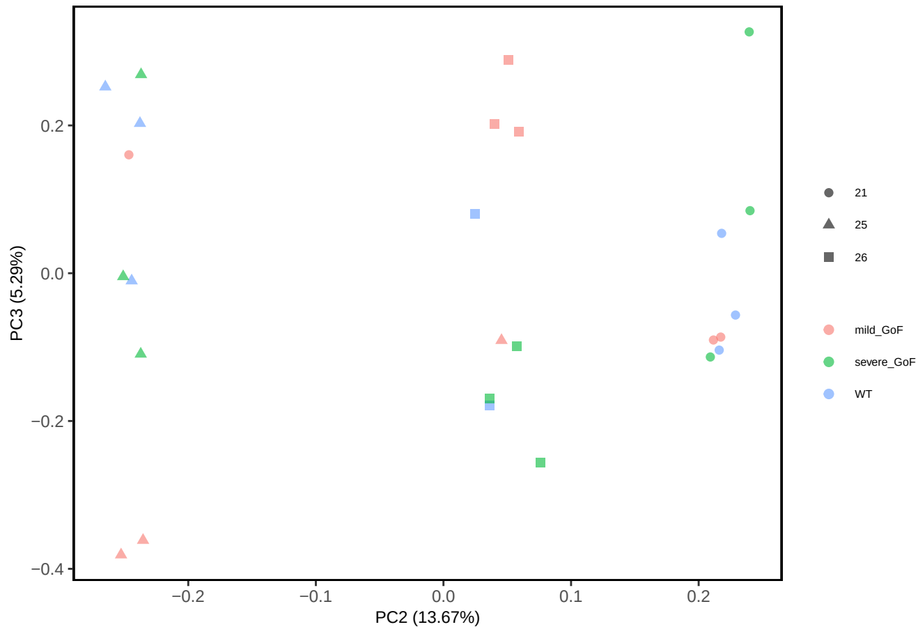
PCA 2 and 3 by Group and Experiment with Batch Effect (Scale = True)
