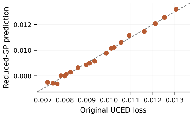
2021 | test R^2 = 0.993
