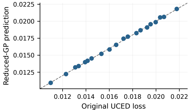
2016 | test R^2 = 0.999
