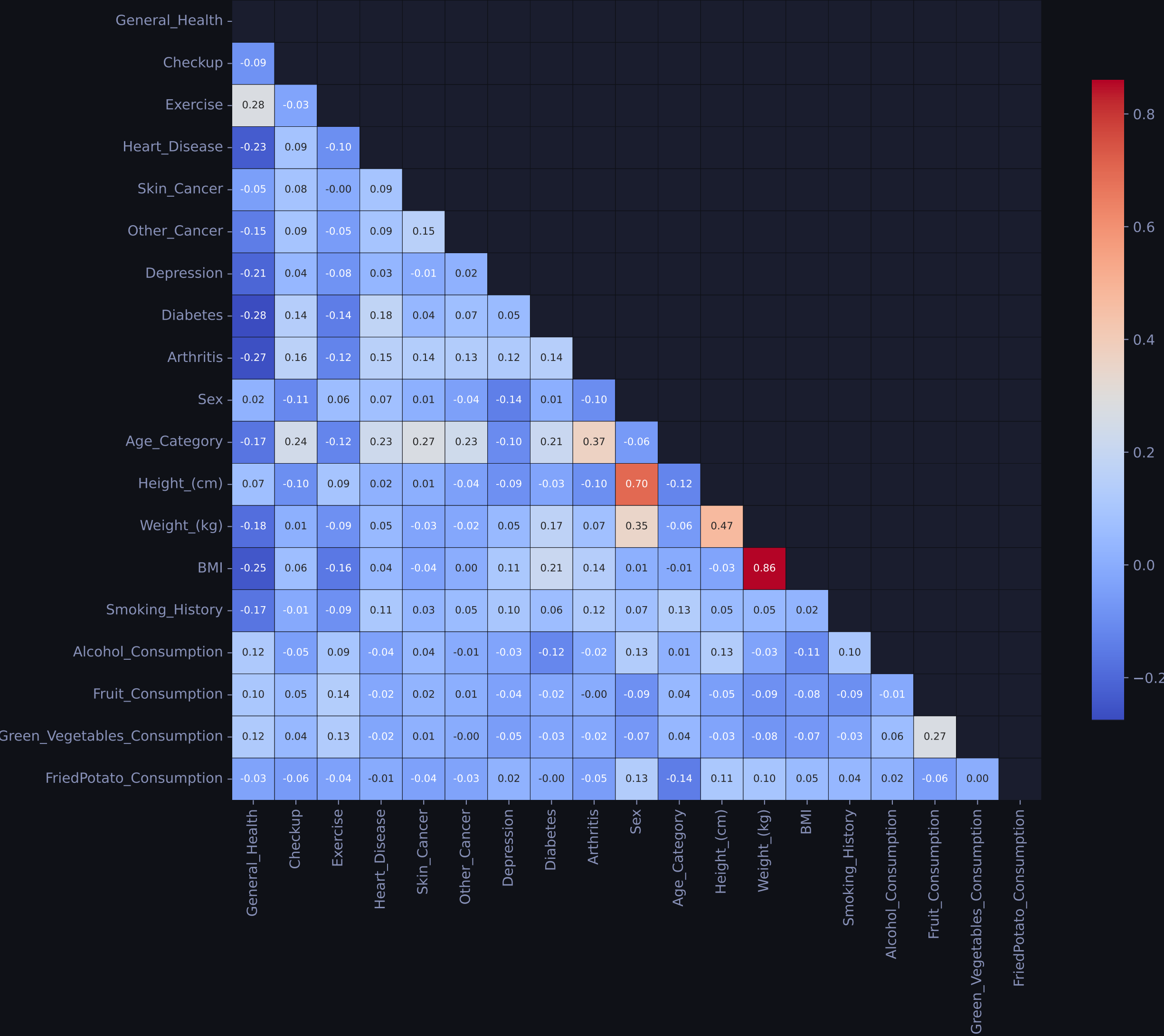
Feature Correlation Matrix
