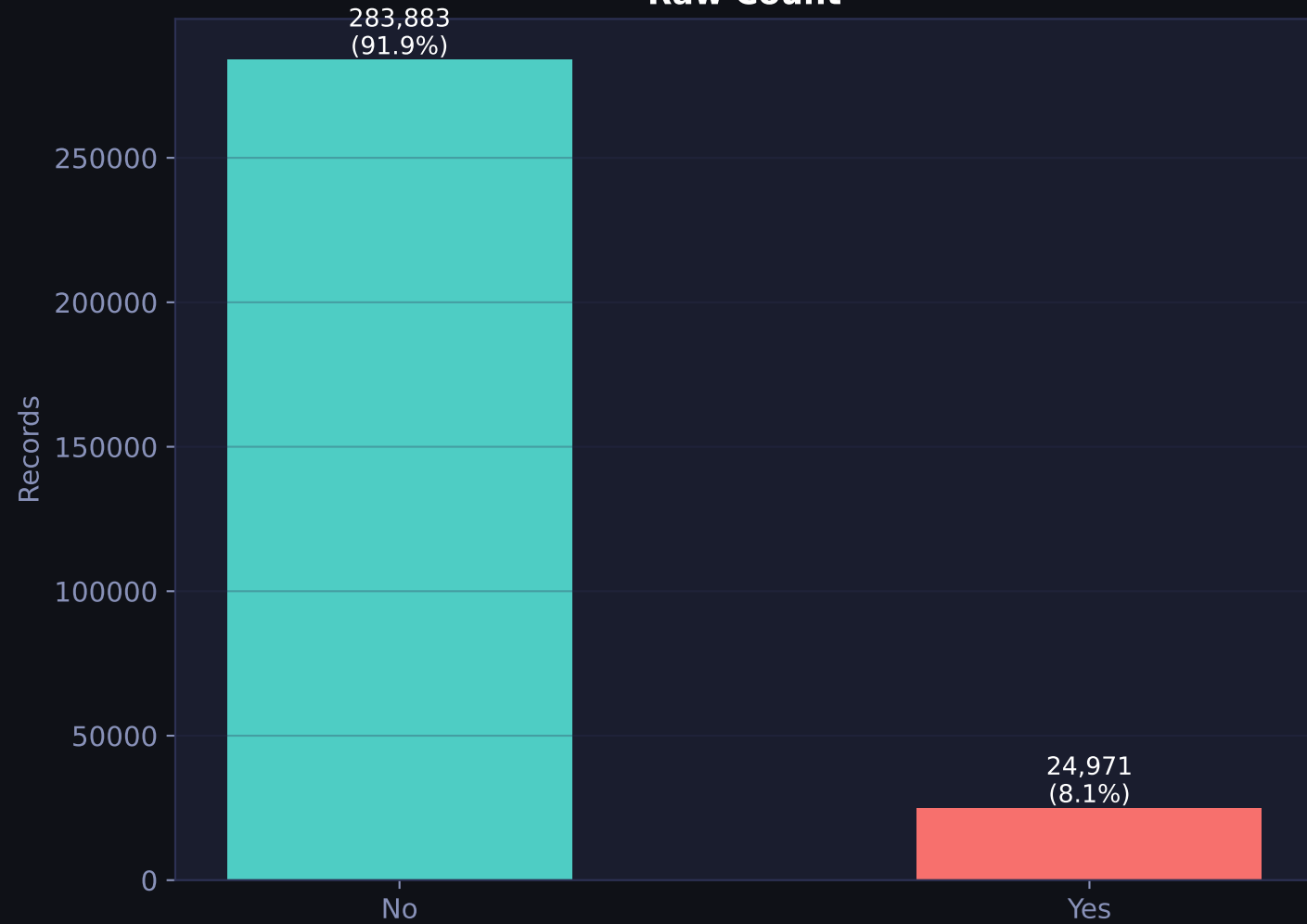
Raw Count
