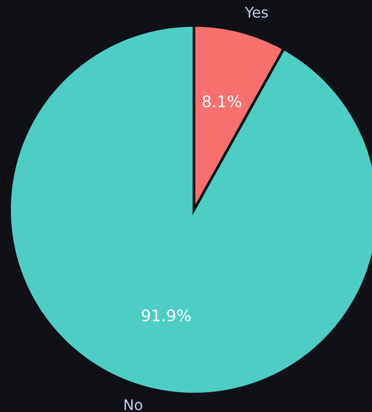
Class Proportion
