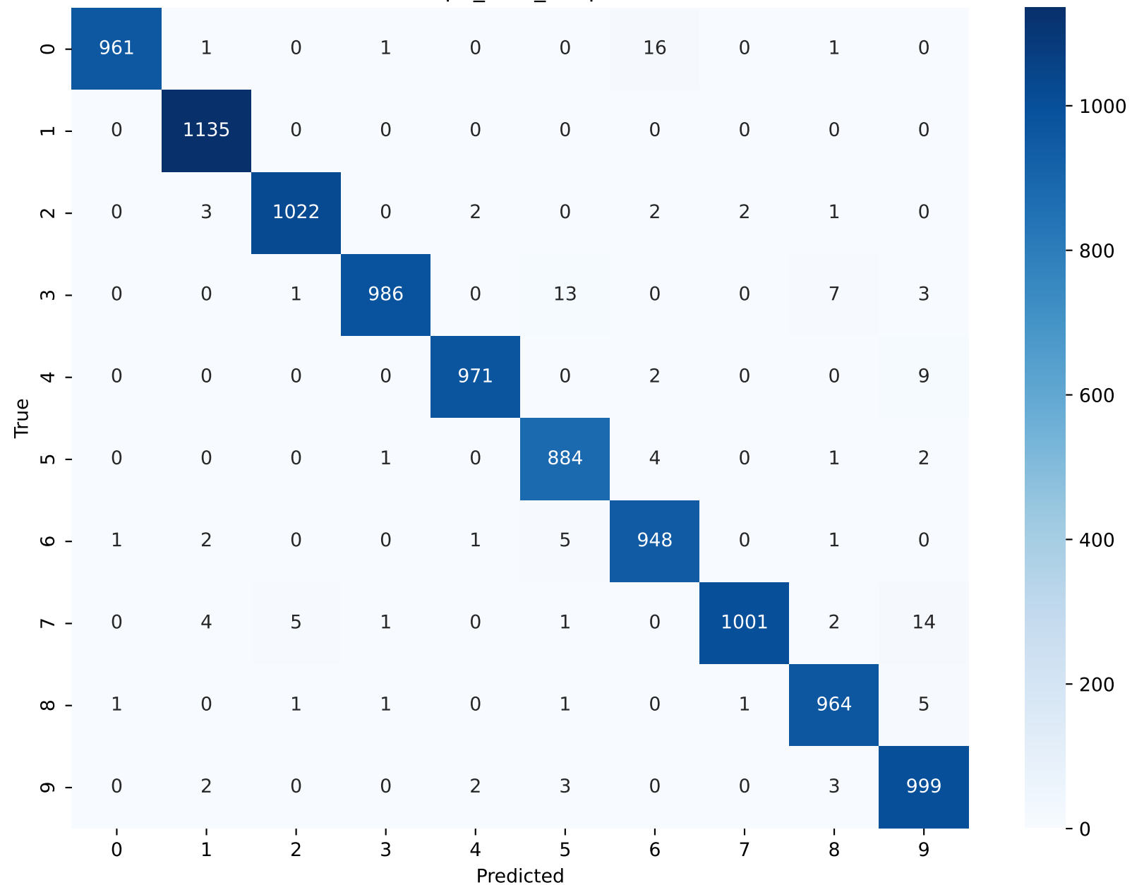
exp1_CNN_Simple
